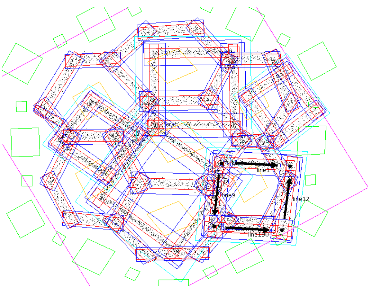
Figure 6: a fourth square found by the program.
