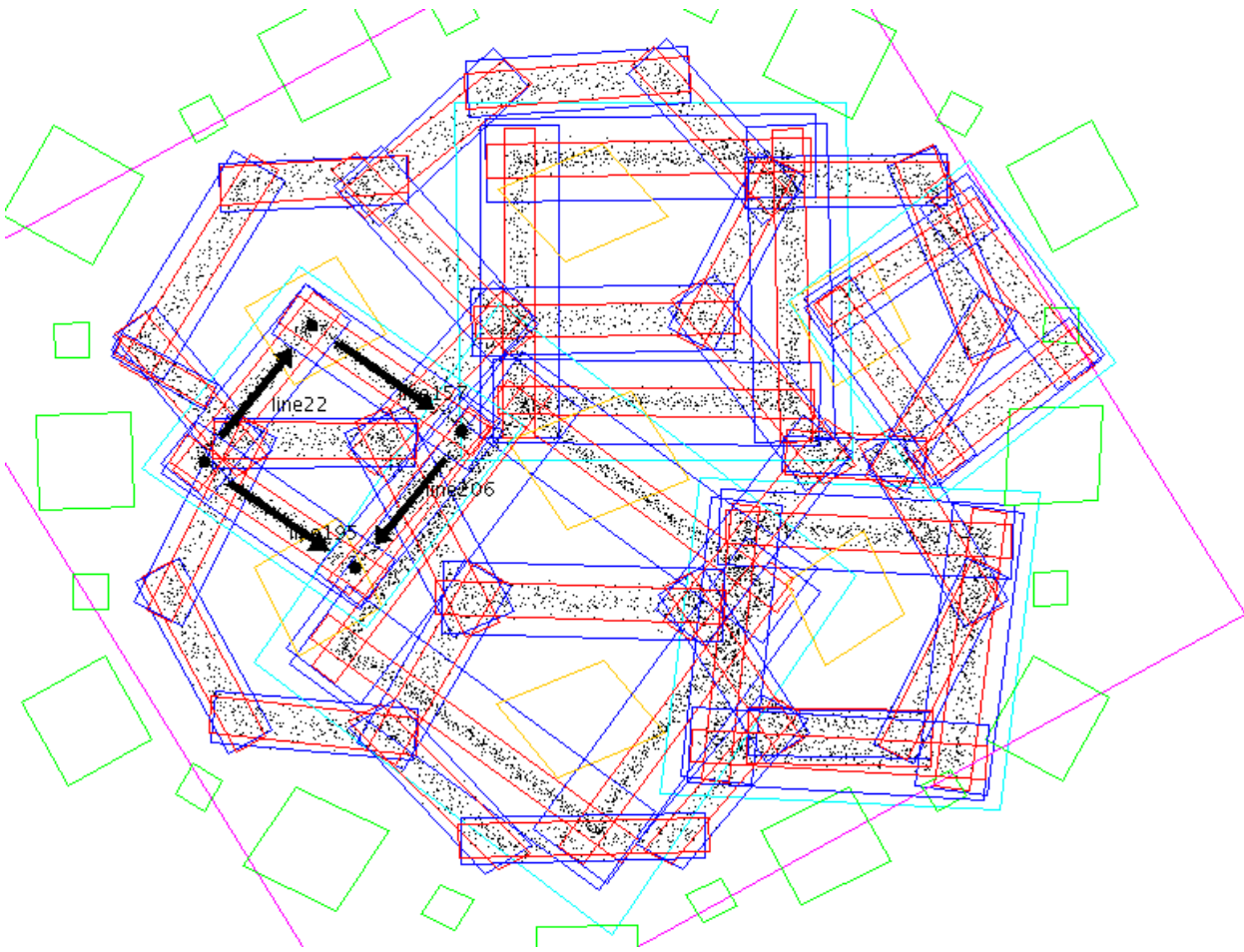
Figure 3: one square found by the program.
