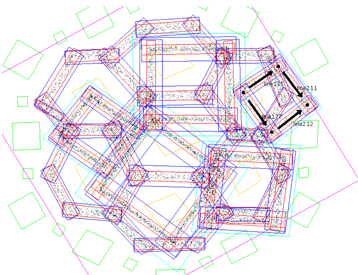
Figure 7: a fifth square found by the program.
