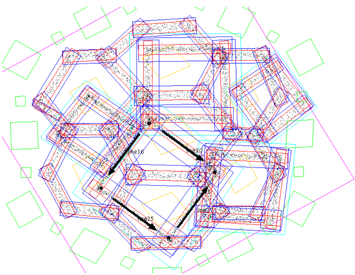
Figure 5: a third square found by the program.
