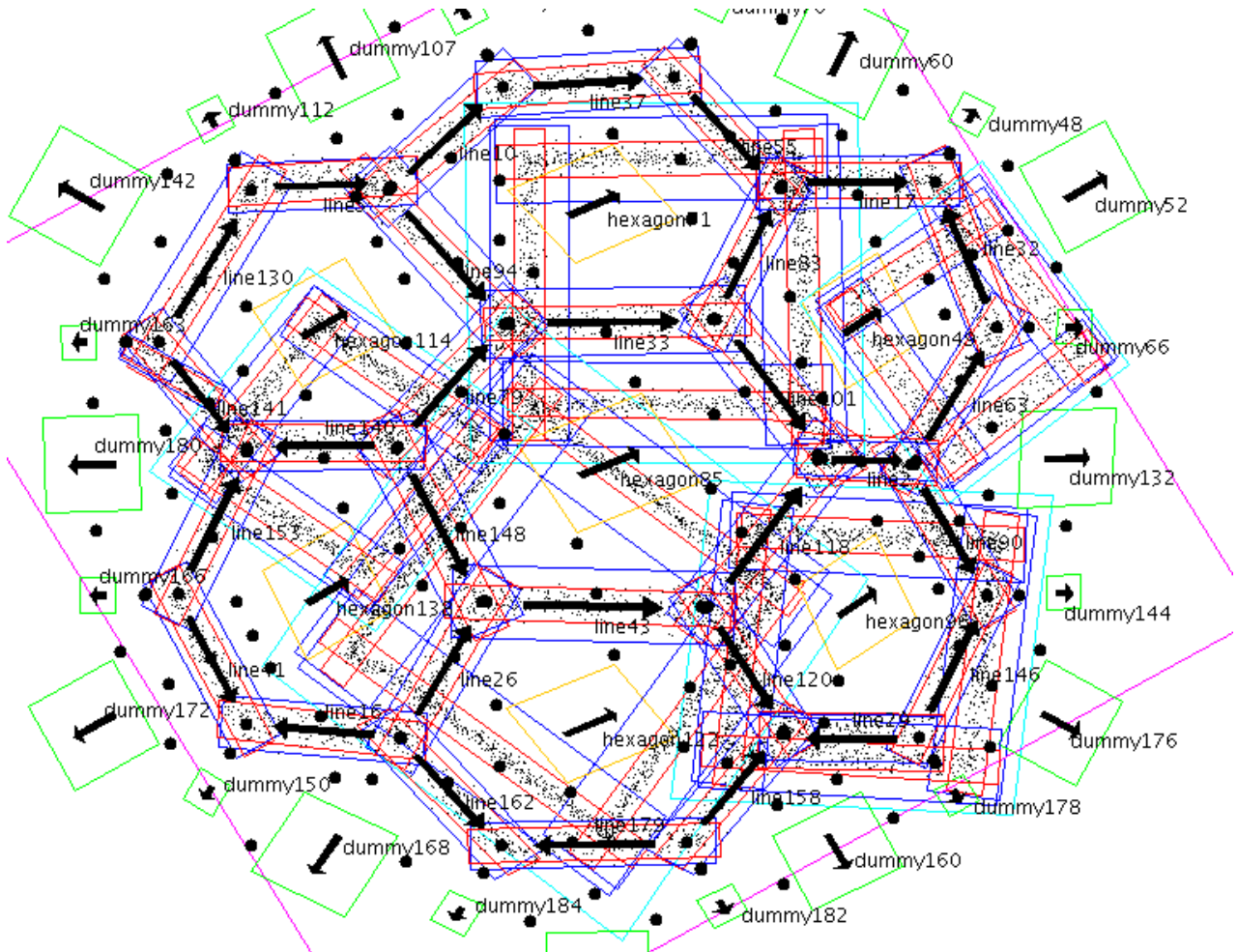
Figure 2: the hexagonal tessellation found by the program.
