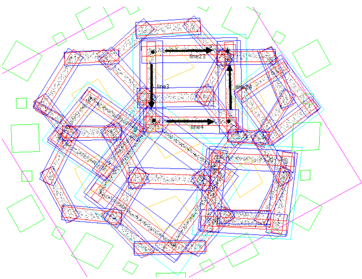
Figure 4: another square found by the program.
